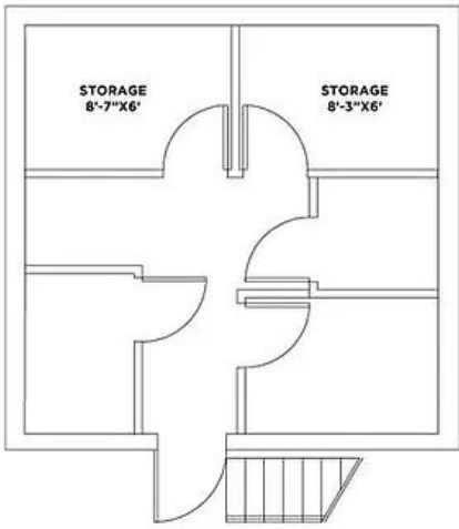
BASEMENT FLOOR
