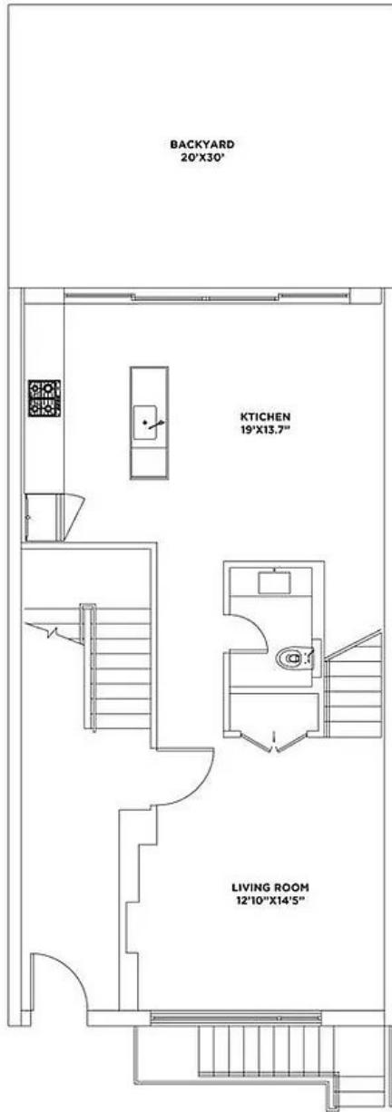
FIRST FLOOR
